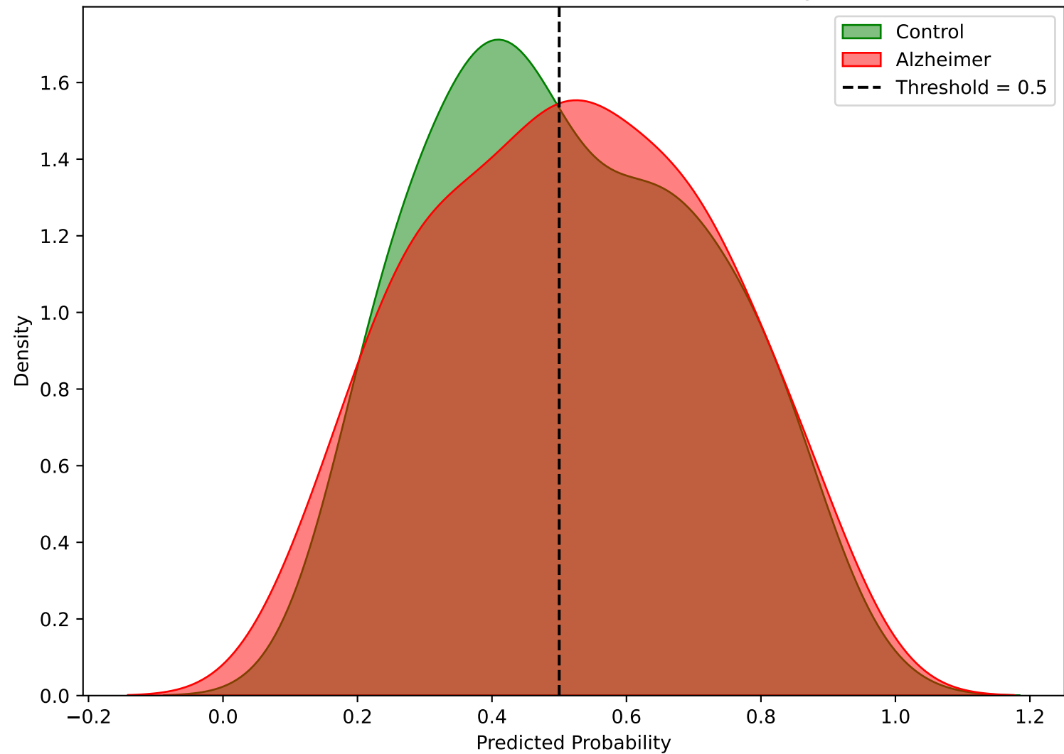
Risk Score Distribution - GradientBoosting
